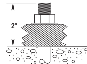
ANCHOR BASE DETAIL
