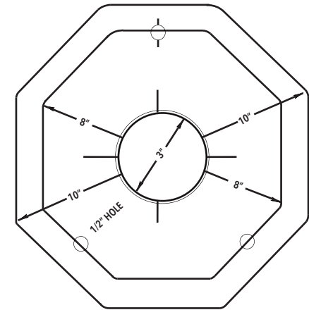
ANCHOR BASE DETAIL
