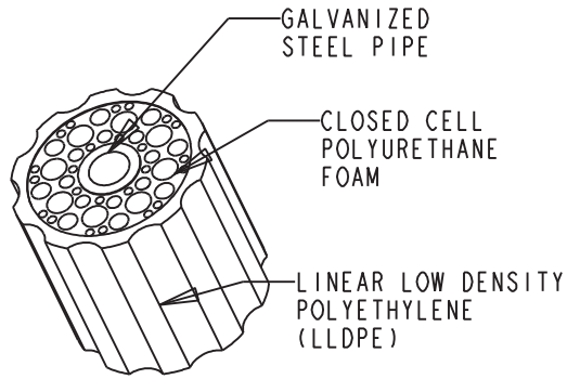
POLYSTEEL PIPE
