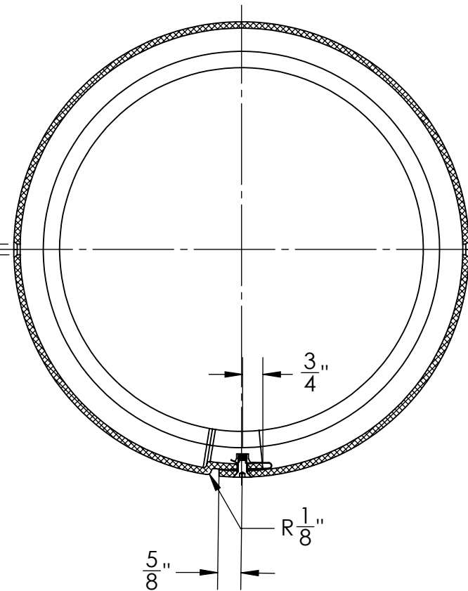
SECTION F-F
