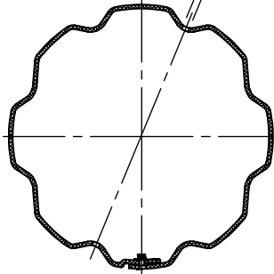
SECTION E-E
