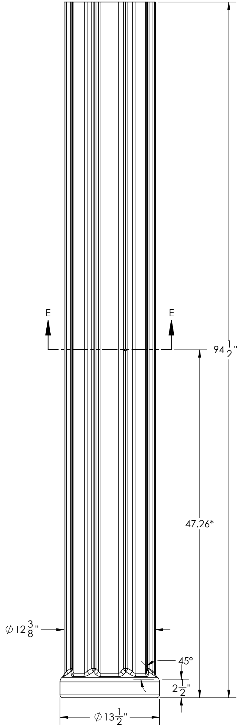
FRONT VIEW
