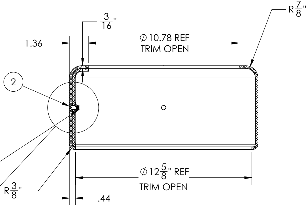
SECTION G-G
